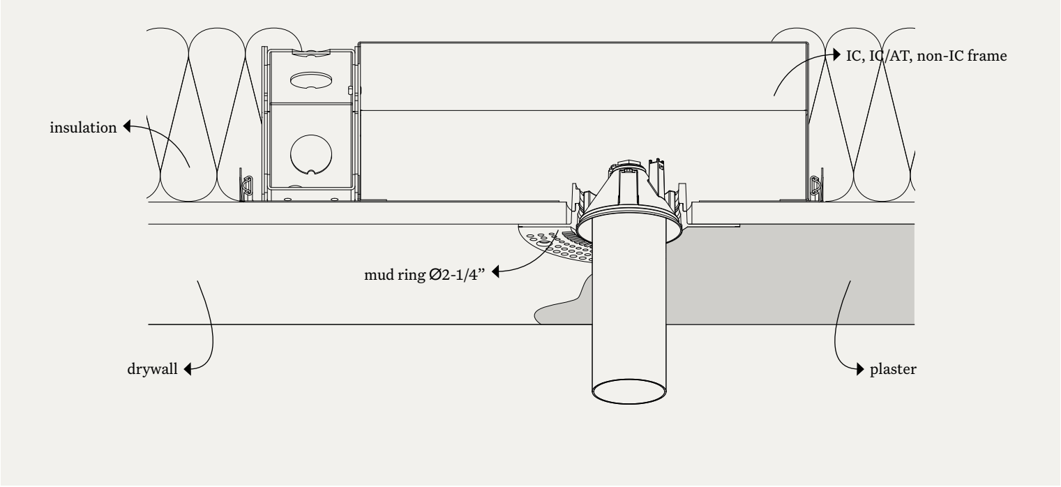
mud ring Ø2-1/4" (Ø57 mm)
