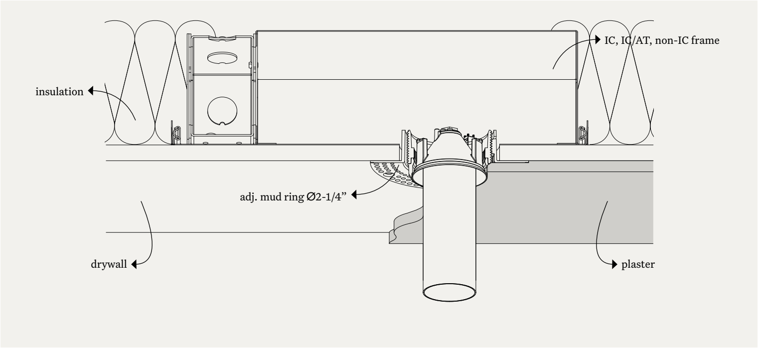
adj. mud ring Ø2-1/4" (Ø57 mm)
