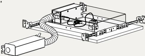
new construction IC 2-1/4"
